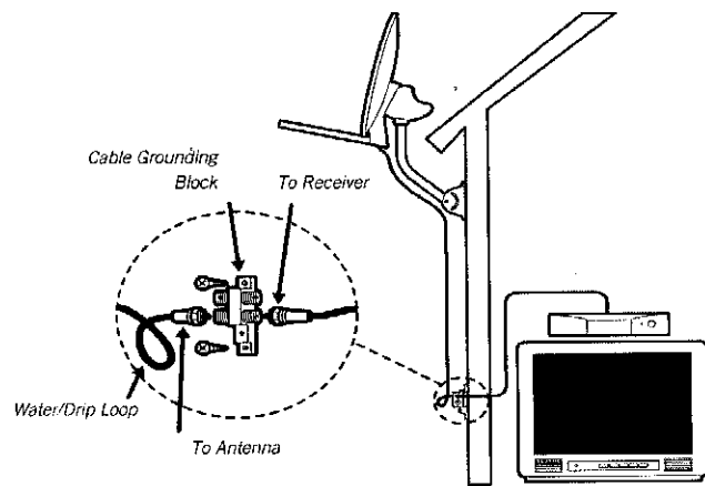
Dual grounding block, one receiver hook up shown
